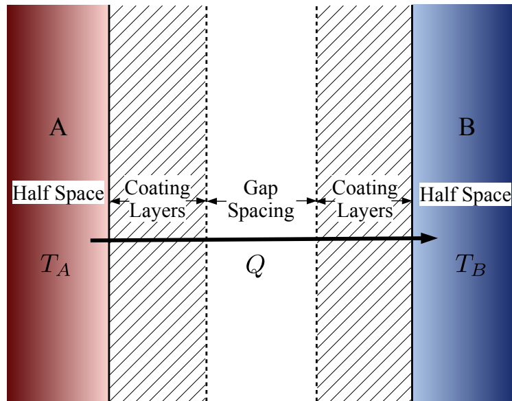
Figure 1.1: Two half-spaces separated by a series of material coating layers and vacuum gaps carriers in both half-spaces. Moreover, the thin layers and gaps affect the way the energy transfers through the layers into the other domain. One such example of a multilayered structure is shown in Fig. 1.1.
