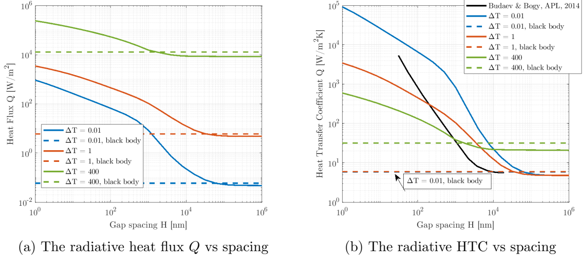
Figure 7.2: The radiative heat flux between two half-spaces A and B with known T_A and T_B using the unified radiation field approach vs spacing in solid lines, identical material are used for A and B with speed c_A = c_B = 0.45c_0 , the dotted lines show the black body radiation (BBR) results
