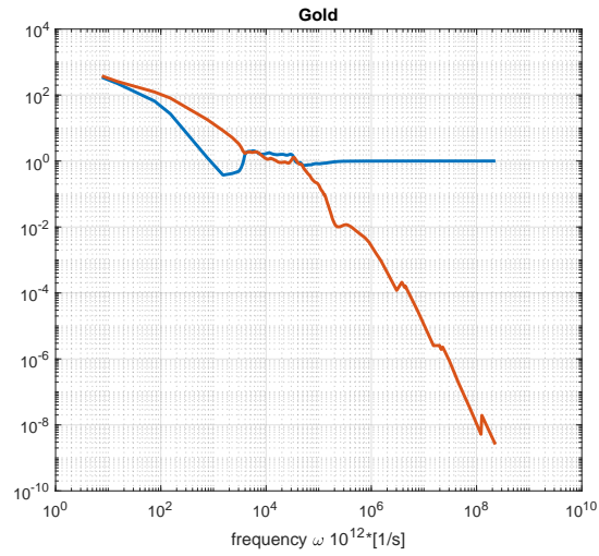
Figure 8.2: The complex refractive ( n' ) index and extinction coefficient ( n'' ) as a function of frequency for gold (blue curve: n' , red curve: n'' ) [69]
