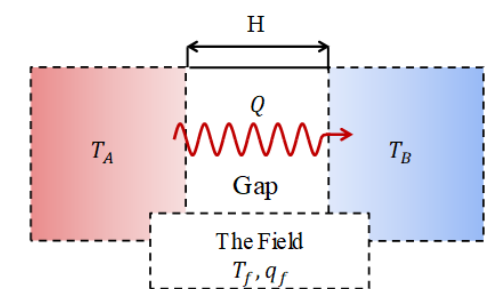
Figure 7.1: Two half-space with a unified emission field which is present in the entire media and describe the distribution of the emission in both half-spaces
