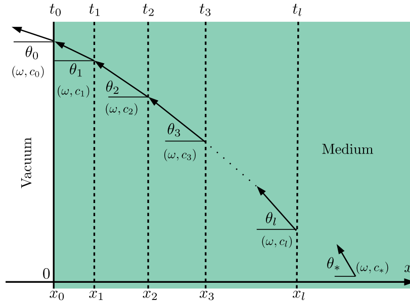
Figure 6.2: The path of a wave or photon in an absorbing material from the origin until exit we compute the heat flow during the time \Delta t to obtain the set \mathbb{I}(\omega, \theta_0, \Delta t) . Eventually, an integration over all (\omega, \theta_0) determines the total heat transfer to the vacuum.
