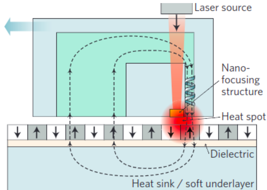
Figure 2.2: The HAMR HDI schematic [40]
